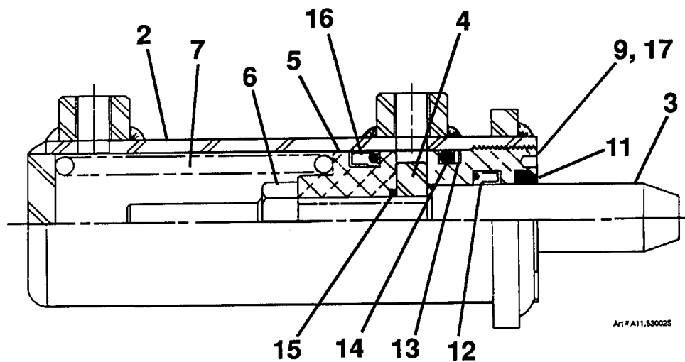
Brake Cylinder Internal Components (Type 2 Cylinder shown)
